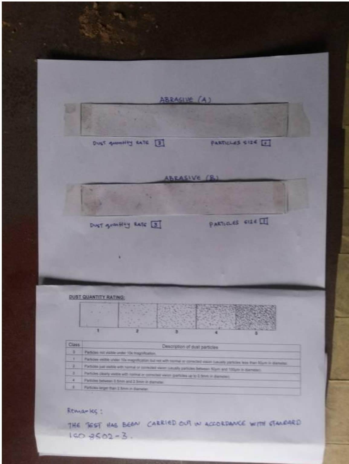
THE VIEW OF RESULT DUST LEVEL TEST
